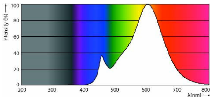
Spectral Power Distribution Colour - LED classic 25W T25L E14 CL ND RF SRT4
