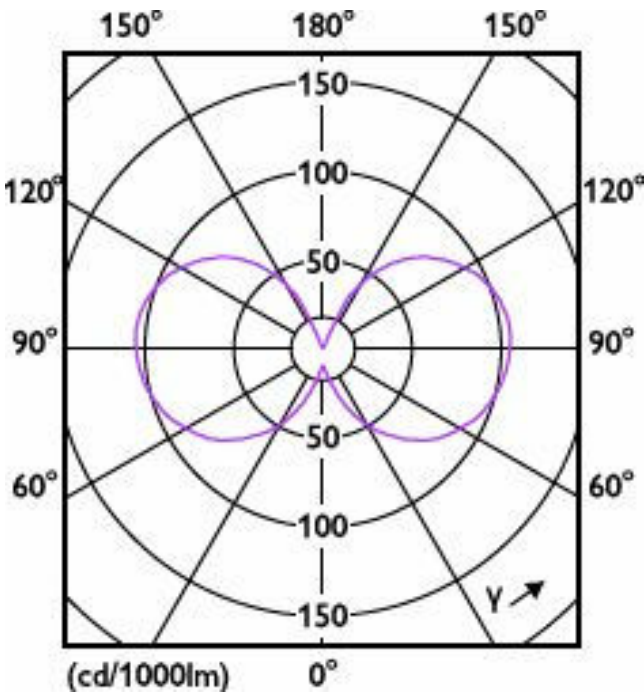
Light Distribution Diagram - LED classic 25W T25L E14 CL ND RF SRT4
