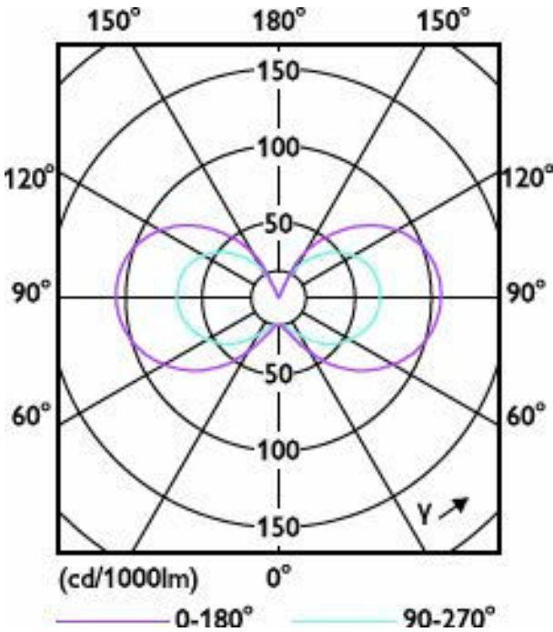
Light Distribution Diagram - CorePro LEDcapsuleLV 1.8-20W GY6.35 827
