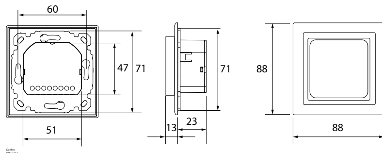
Figur: Danfoss Icon2™ / 24 V RT rumtermostat 088U2128
