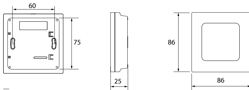
Figur: Danfoss Icon2™ / 24 V RT rumtermostat 088U2128
