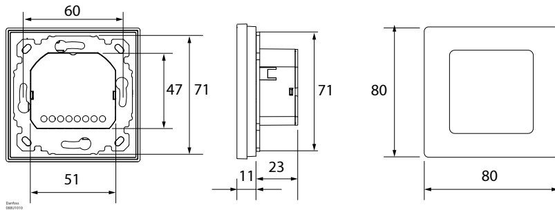
Figur: Danfoss Icon2™ / 24 V RT rumtermostat 088U2126
