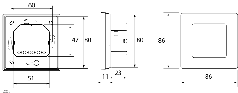
Figur: Danfoss Icon2™ / 24 V RT rumtermostat 088U2127
