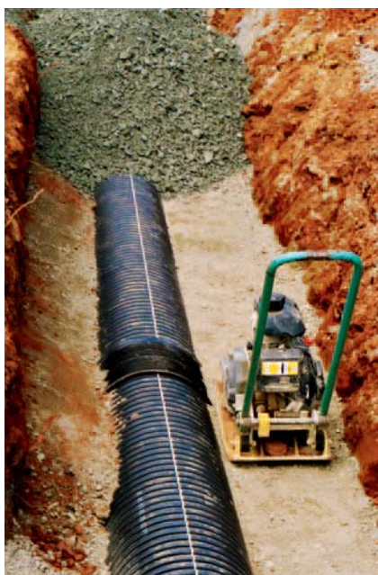
SIROPLAST-K multi-purpose pipes for combined discharge of drainage and surface water
