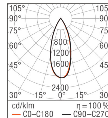
SPOT LED 68 7 W IP65 FP WT
