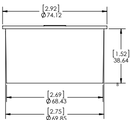
HOUSING (NO GASKET)
