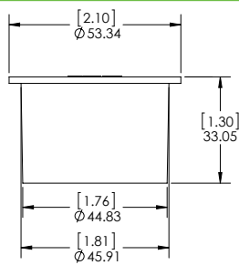
HOUSING (NO GASKET)
