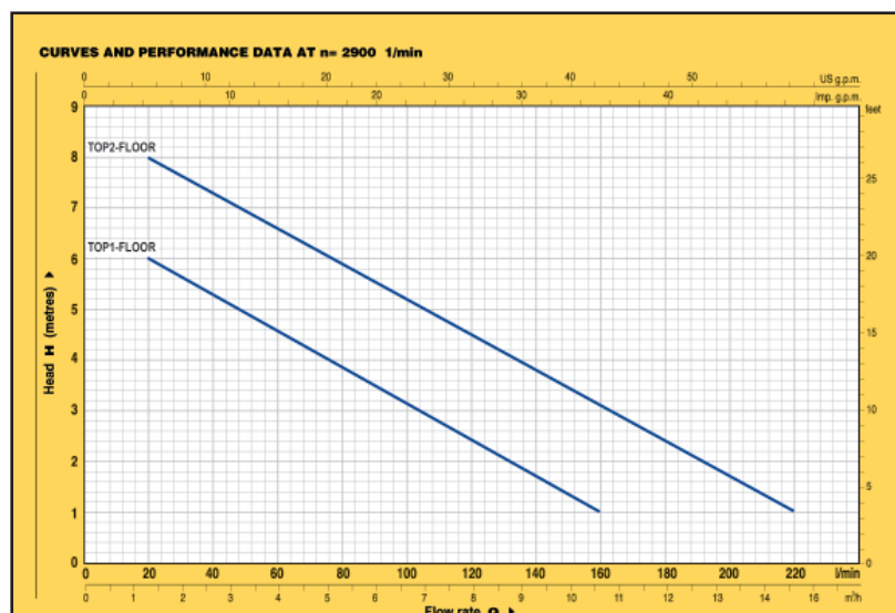
Pumpekurve
