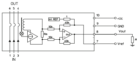
Figure 21: Test connection
