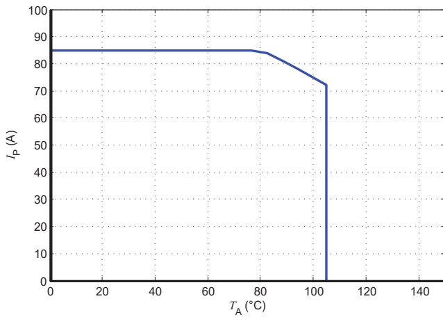
Figure 18: I_p vs T_A for LXSR 25-NPS
