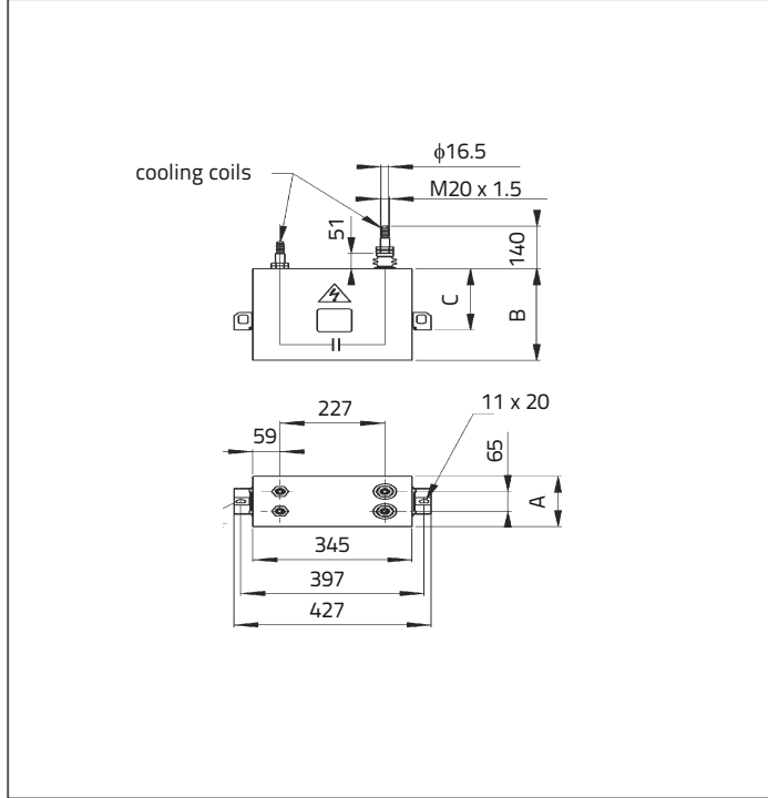
Picture 5 - KLS x200 Double Cooling Coils Capacitor - "live" case
