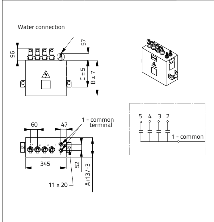
Picture 3 - KLS x2xx Single Cooling Coil Capacitor ("Live" Case)Hz
