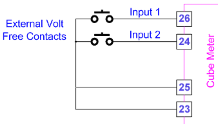
Figure 1-1 Input Connection
