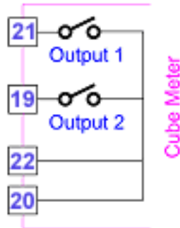
Figure 2-1 Output Schematic (Shown in auxiliary power off state)
