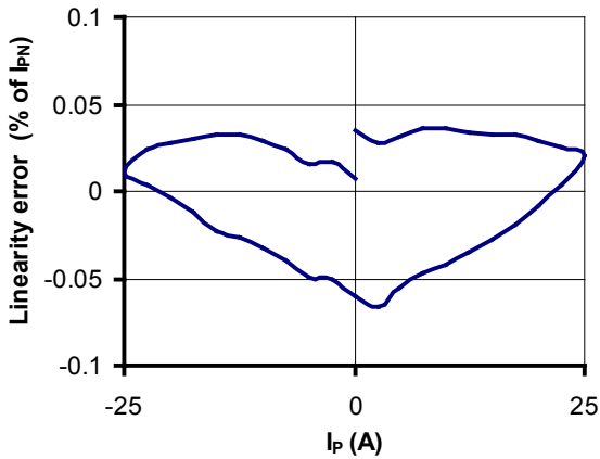
Figure 13: Linearity error
