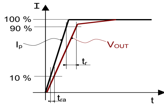
Figure 31: Response time t_r and reaction time t_{ra}
