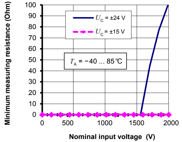
Figure 2: Minimum measuring resistance The derating @ ±24 is only applicable for T_A = 80 \text{ °C} \dots 85 \text{ °C} For T_A under 80 \text{ °C} , the minimum measuring resistance is 0 \text{ }\Omega whatever U_C
