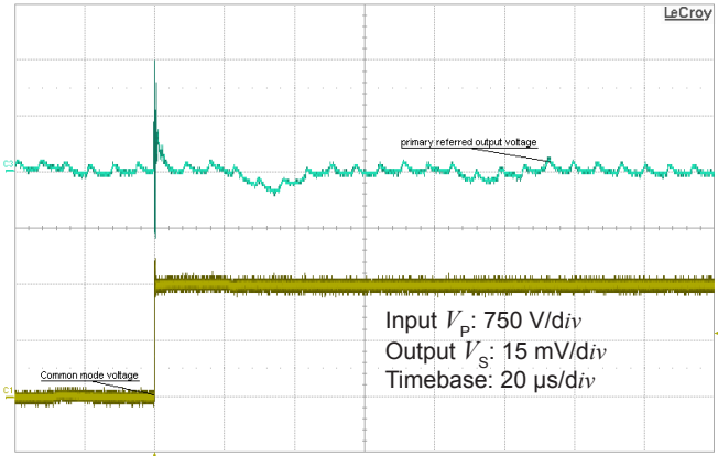
Figure 10: Detail of typical common mode perturbation (1500 V step with 6 kV/μs, R_M = 100 \text{ k}\Omega )
