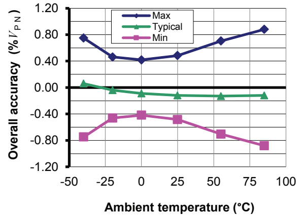
Figure 2: Overall accuracy in temperature
