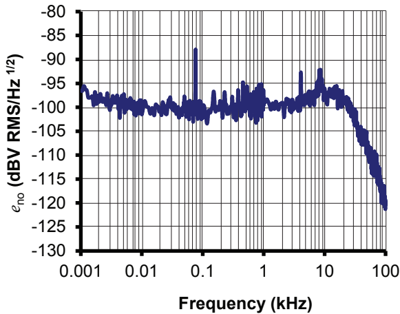
Figure 11: Typical output RMS noise voltage spectral density e_{no} with R_M = 2 \text{ k}\Omega
