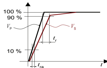
Figure 15: Response time t_r and reaction time t_{ra}
