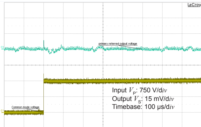
Figure 9: Typical common mode perturbation (1500 V step with 6 kV/μs R_M = 100 \text{ k}\Omega )
