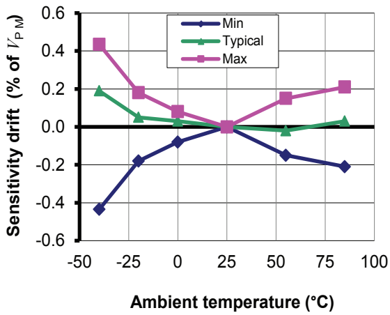
Figure 3: Sensitivity thermal drift
