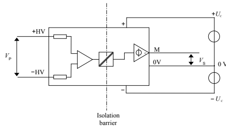
Figure 14: Standard characterization schematics for voltage output transducers ( R_M = 100 \text{ k}\Omega unless otherwise noted)
