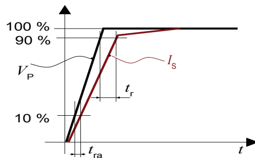
Figure 17: Response time t_r and reaction time t_{ra}
