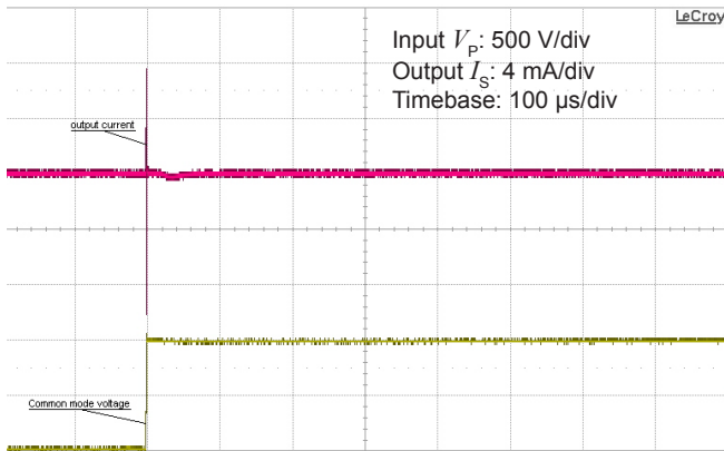
Figure 11: Typical common mode perturbation (1000 V step with 6 kV/μs, R_M = 100 \Omega )
