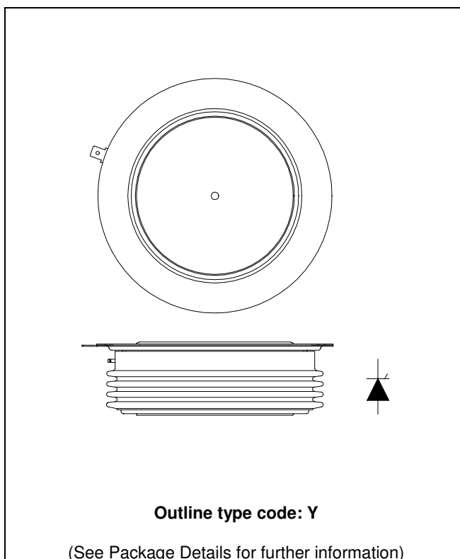
Fig. 1 Package outline
