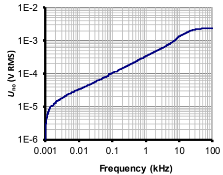
Figure 7: Typical total output RMS noise current U_{no} referred to secondary with RM = 2\text{ k}\Omega
