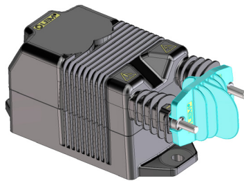
Assembly of UL 347 Isolator on primary studs.
