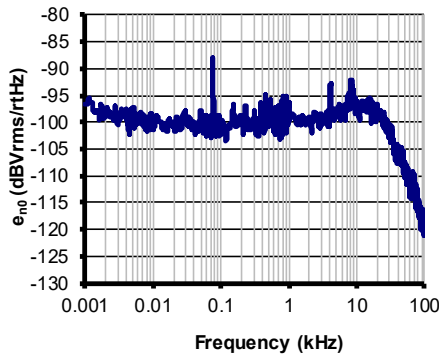
Figure 6: Typical output noise voltage density U_{no} referred to secondary with RM = 2\text{ k}\Omega
