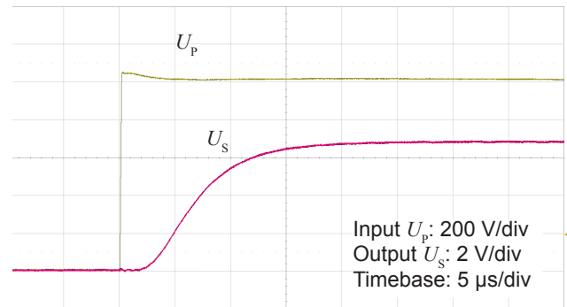
Figure 7: Typical step response (0 to 1000 V)
