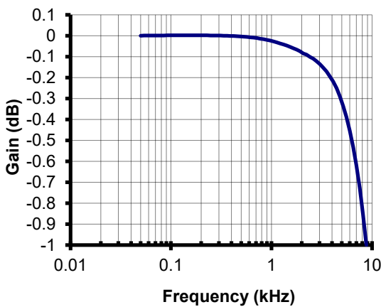
Figure 8: Typical frequency and phase response (detail)
