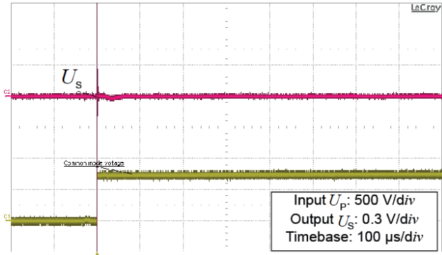
Figure 9: Typical common mode perturbation (750 V step with 6 kV/μs, R_M = 100 \text{ k}\Omega )
