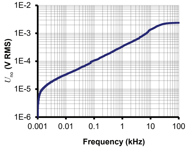
Figure 12: Typical total output RMS noise voltage with R_M = 2 \text{ k}\Omega ( f_c is upper cut-off frequency of bandpass, low cut off frequency is 1 Hz)
