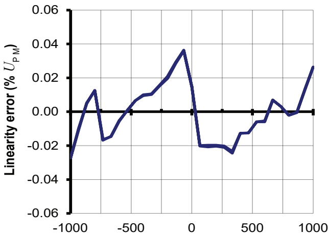
Figure 13: Typical linearity error at 25 °C
