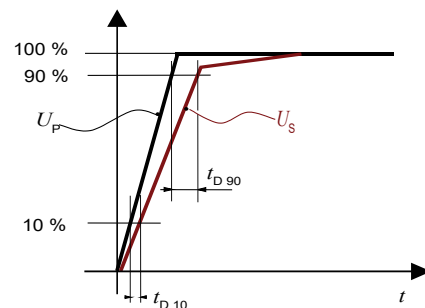
Figure 15: t_{D10} (delay time @ 10 %) and t_{D90} (delay time @ 90 %)
