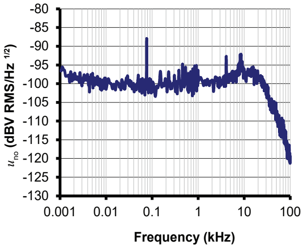
Figure 11: Typical output RMS noise voltage spectral density u_{no} with R_M = 2 \text{ k}\Omega
