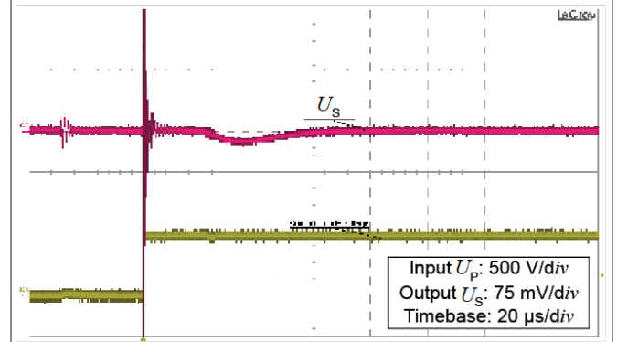
Figure 10: Detail of typical common mode perturbation (750 V step with 6 kV/μs, R_M = 100 \text{ k}\Omega )
