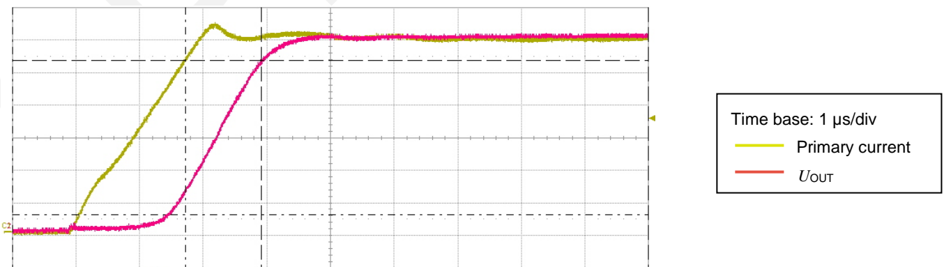
Figure X di/dt
