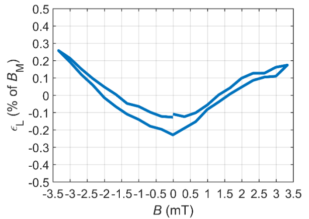
Figure X Linearity error @125 °C
