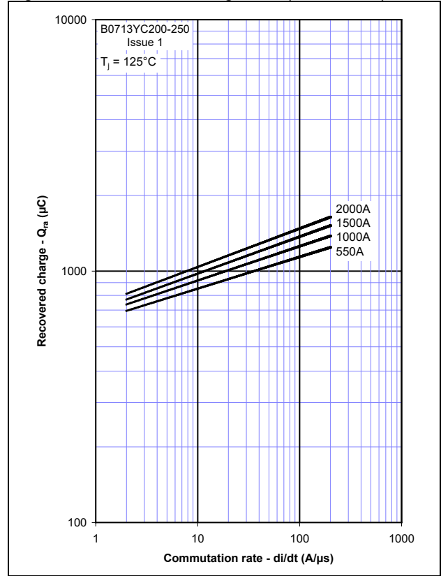
Figure 6 - Recovered charge, Q_{ra} (50% chord) (µC)
