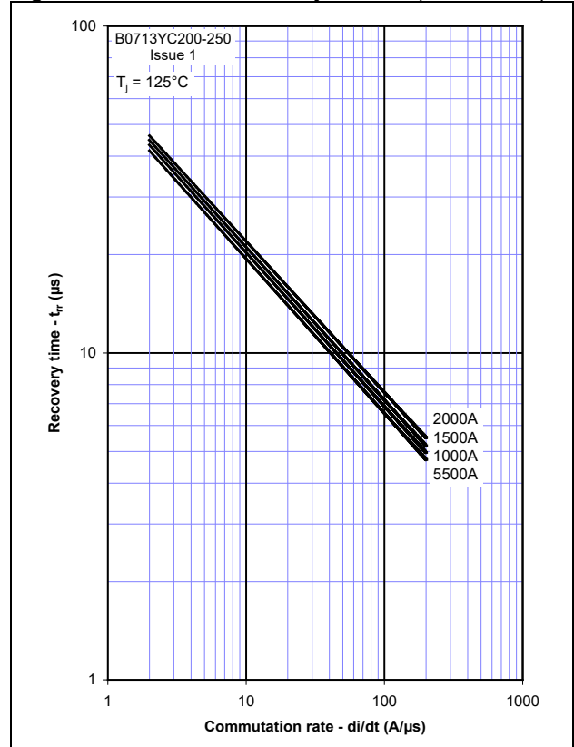
Figure 8 - Maximum recovery time, t_{rr} (50% chord) (µs)
