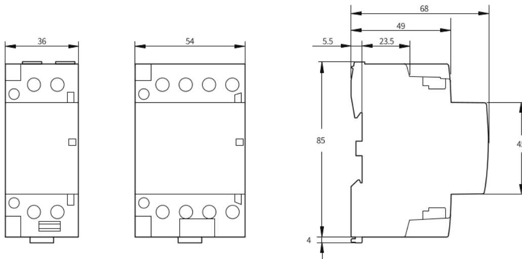
FPC1 -32A-63A
