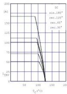
Fig.5 Maximum forward current at case temperature
