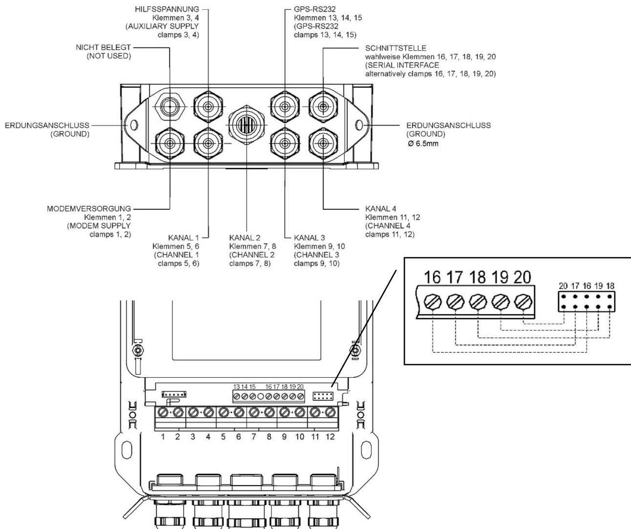
Figure 3.2: Terminal block
