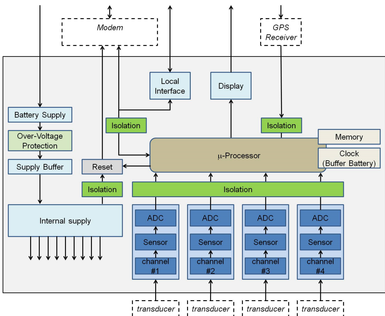
Figure 2.1: Block diagram
