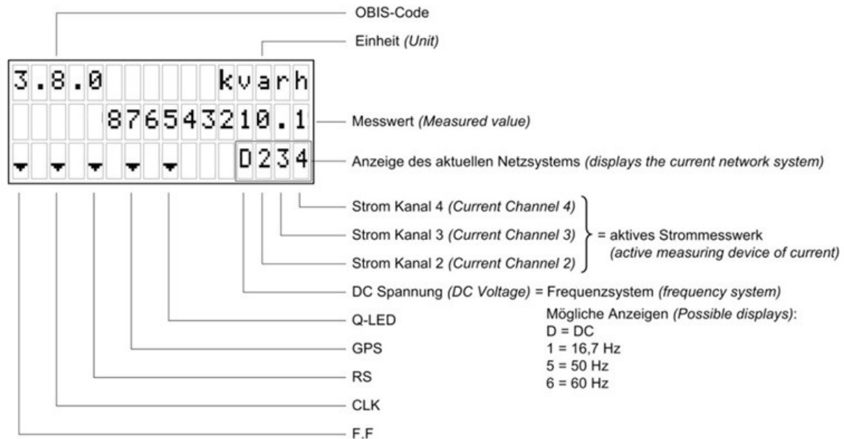
Figure 4.1: LC display
