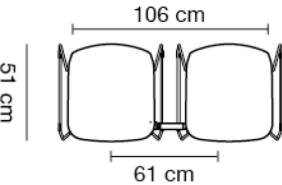
Pato Sledge Chair Base coupling
