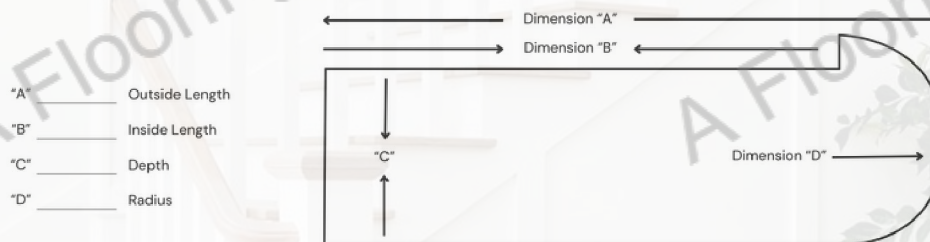
Right Hand Bullnose Starter
