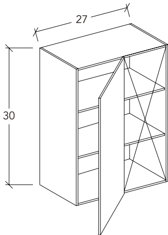
30" HIGH WALL BLIND CORNER CABINET
