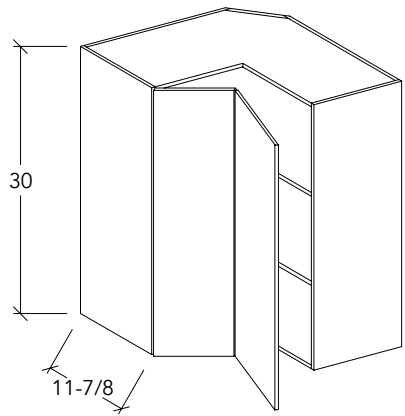
30" HIGH CORNER WALL CABINET
