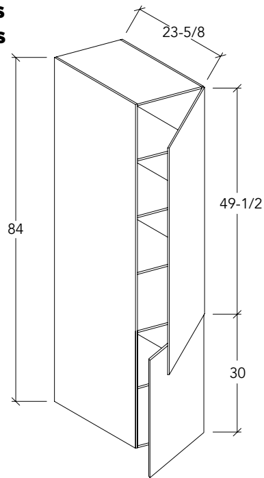
84" HIGH PANTRY WITH TWO DOORS AND FIVE SHELVES
