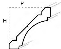
COVE RCRMC Height: 3 1/8" Projection: 3 1/8"
