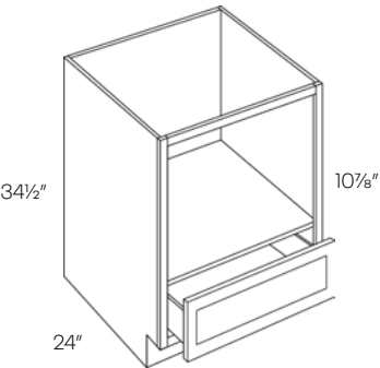
Microwave Base Cabinet
