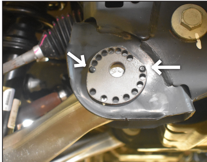
FIGURE C (CAMS CENTERED)
