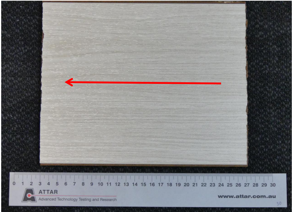
Figure 1: GH 8mm Laminate plank Arrow indicates direction of testing
