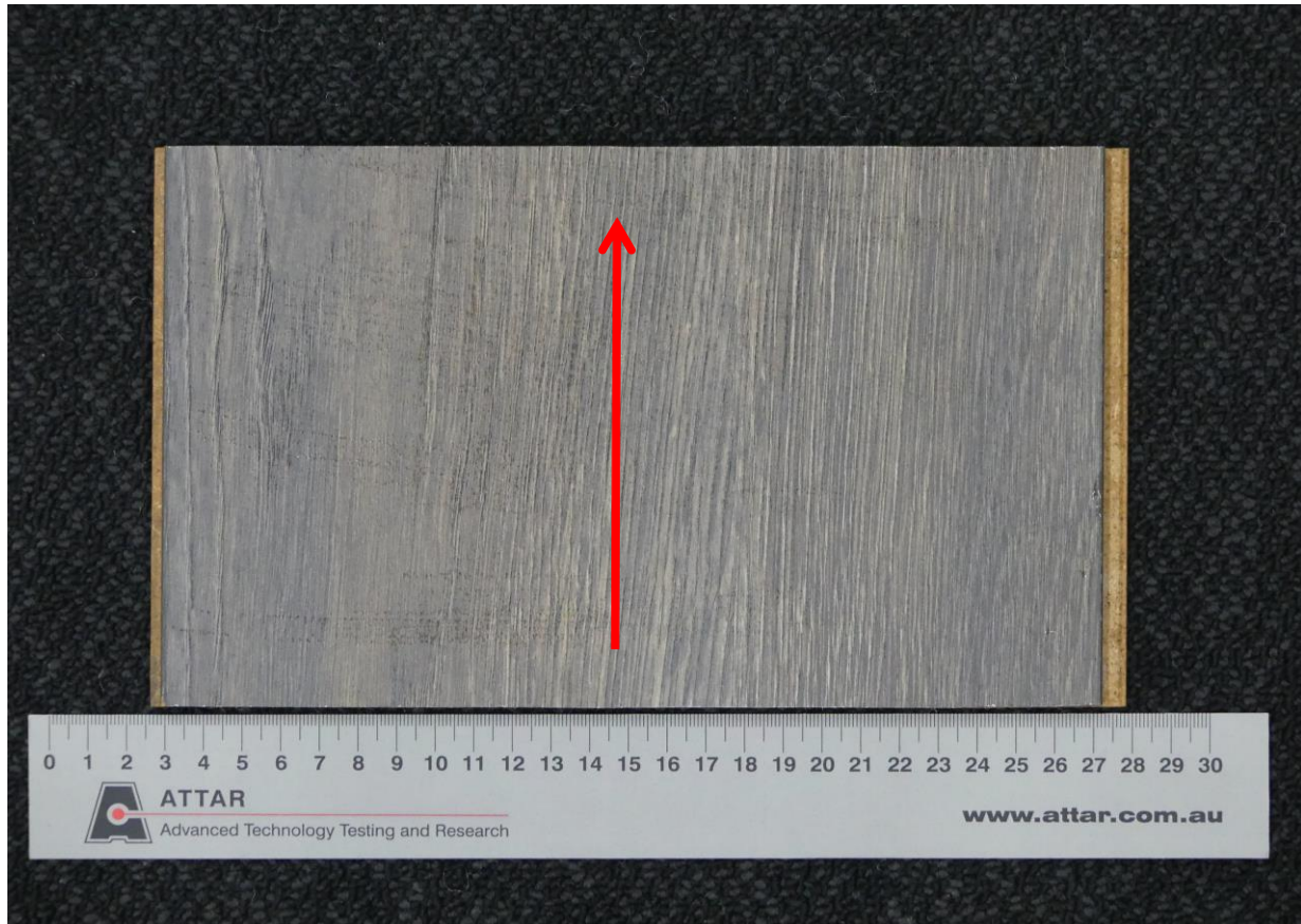
Figure 1: Photo of the specimen tested. Arrow indicates direction of testing
