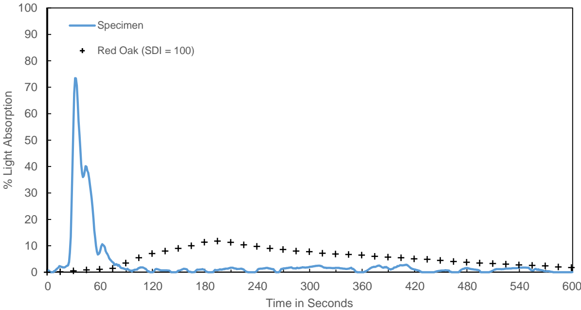
Chart 2. SMOKE DEVELOPED
