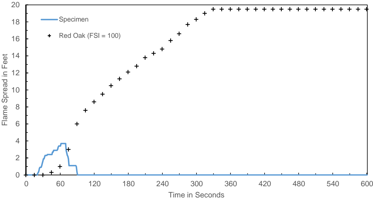
Chart 1. FLAME SPREAD
