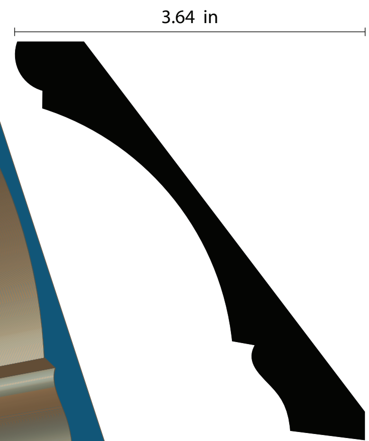
CN-031 .75" x 5.562"
