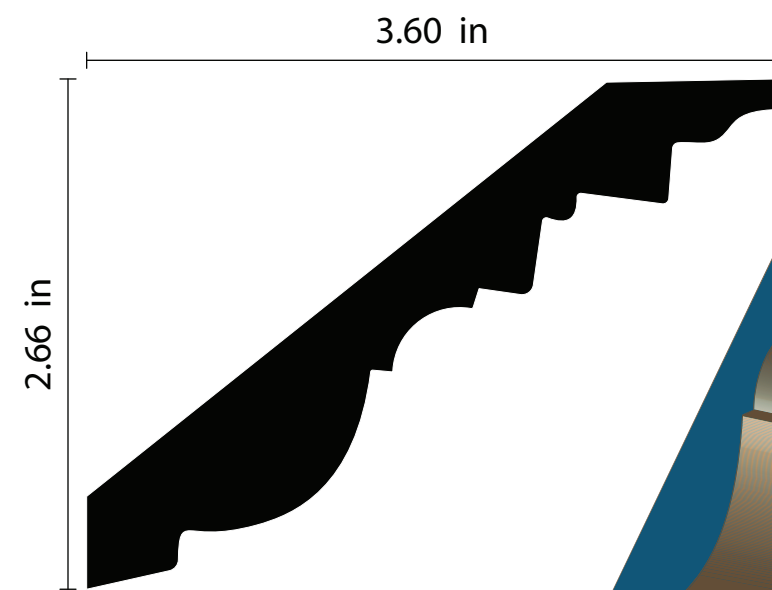
CN-030 .75" x 4.5"
