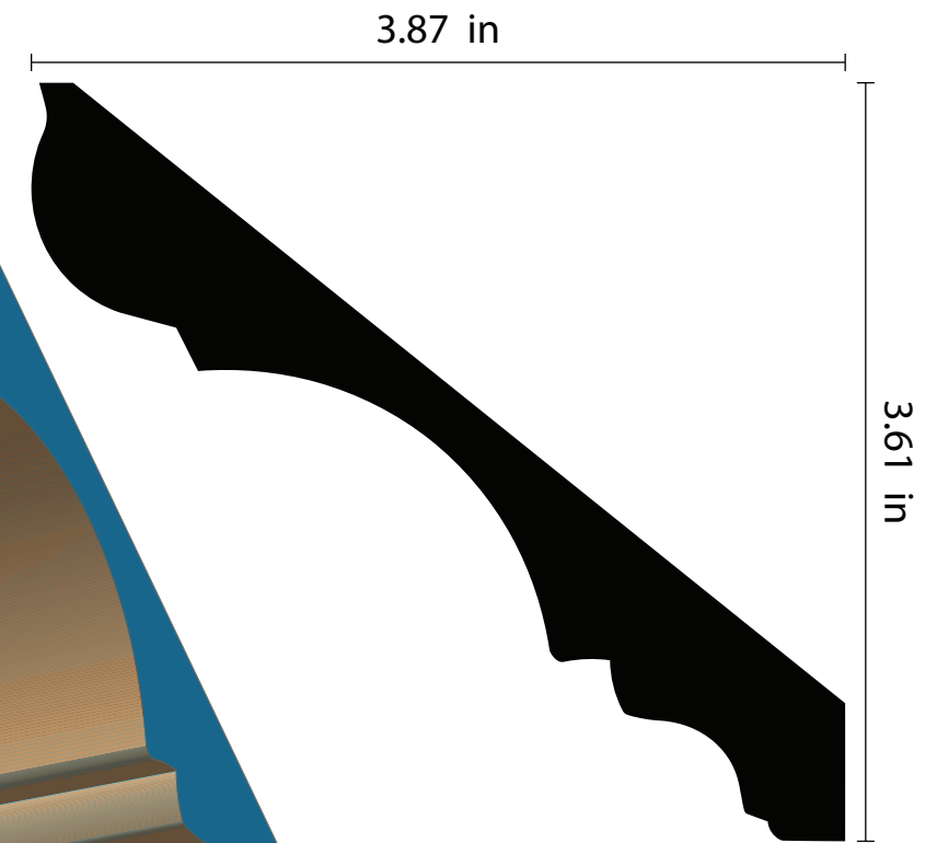
CN-037 .75" x 5.25"
