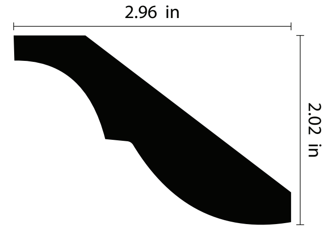
CN-038 .75" x 3.562"
