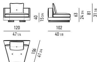
LOW ELEMENTO CENTRALE SIMMETRICO THEATRE CM 120 LOW THEATRE SYMMETRICAL CENTRAL ELEMENT CM 120
