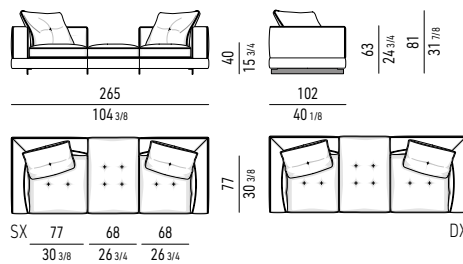
LOW DIVANO ANGOLARE OPEN CM 265 LOW CORNER OPEN SOFA CM 265
