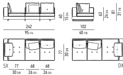
LOW ELEMENTO ANGOLARE DAYBED CM 242 LOW CORNER DAYBED ELEMENT CM 242
