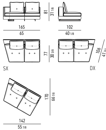
LOW ELEMENTO CENTRALE ASIMMETRICO THEATRE CM 165 LOW THEATRE ASYMMETRICAL CENTRAL ELEMENT CM 165
