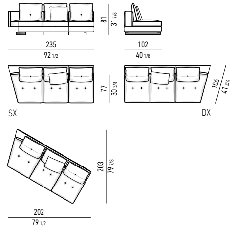
LOW ELEMENTO CENTRALE ASIMMETRICO THEATRE CM 235 LOW THEATRE ASYMMETRICAL CENTRAL ELEMENT CM 235
