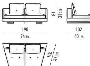
LOW ELEMENTO CENTRALE SIMMETRICO THEATRE CM 190 LOW THEATRE SYMMETRICAL CENTRAL ELEMENT CM 190
