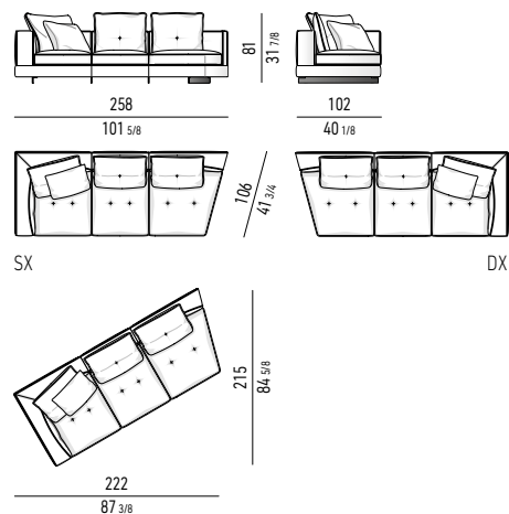
LOW ELEMENTO TERMINALE THEATRE CM 258 LOW THEATRE ELEMENT WITH 1 ARMREST CM 258
