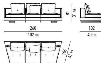
LOW ELEMENTO CENTRALE SIMMETRICO THEATRE CM 260 LOW THEATRE SYMMETRICAL CENTRAL ELEMENT CM 260
