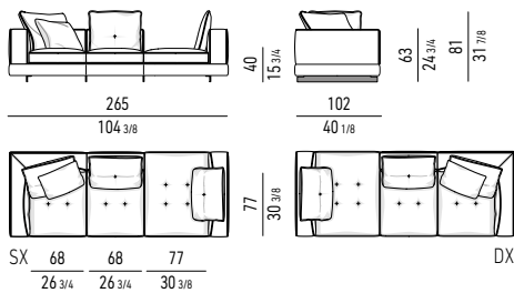
LOW DIVANO ANGOLARE DAYBED CM 265 LOW CORNER DAYBED SOFA CM 265
