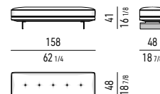
POUF CM 158X48 OTTOMAN CM 158X48
