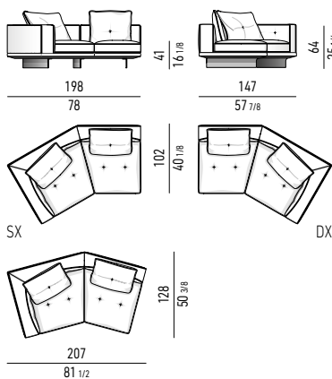
ELEMENTO TERMINALE INCLINATO CM 198X147 INCLINED ELEMENT WITH ARMREST CM 198X147
