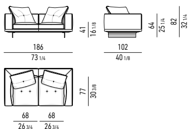
DIVANO CM 186 SOFA CM 186
