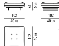
POUF CM 102X102 OTTOMAN CM 102X102
