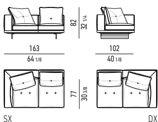
ELEMENTO TERMINALE CM 163 ELEMENT WITH 1 ARMREST CM 163
