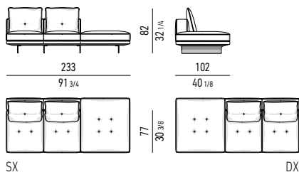
ELEMENTO PENISOLA CM 233 OPEN-END ELEMENT CM 233
