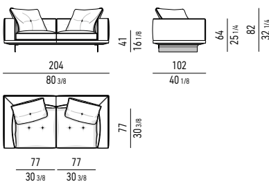
DIVANO CM 204 SOFA CM 204
