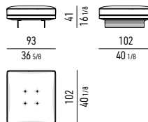
POUF CM 93X102 OTTOMAN CM 93X102
