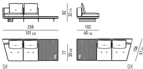
ELEMENTO CENTRALE ASIMMETRICO THEATRE CM 258 CON TOP F THEATRE ASYMMETRICAL CENTRAL ELEMENT CM 258 WITH TOP F
