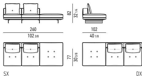
ELEMENTO PENISOLA CM 260 OPEN-END ELEMENT CM 260
