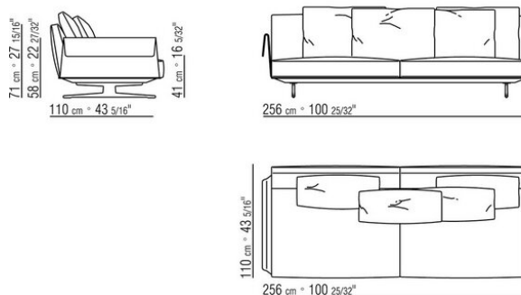
COD. 029017 END UNIT L
