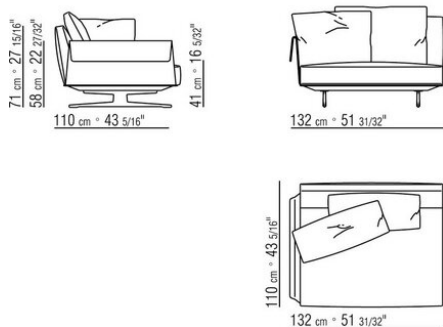
COD. 029015 END UNIT L
