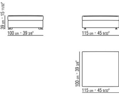
COD. 024399 CUSHION
