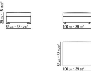
COD. 024398 CUSHION
