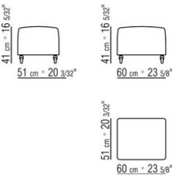
COD. 010953 OTTOMAN W/CASTORS
