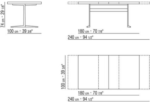
COD. 014X74 TABLE EXTENS.
