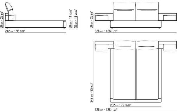
COD. 0243YC BED WITHOUT PLATFORM
