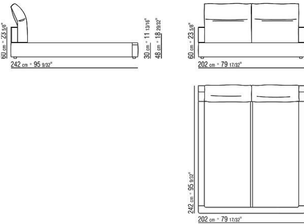
COD. 0243VC SLIM BED WITHOUT PLATFORM
