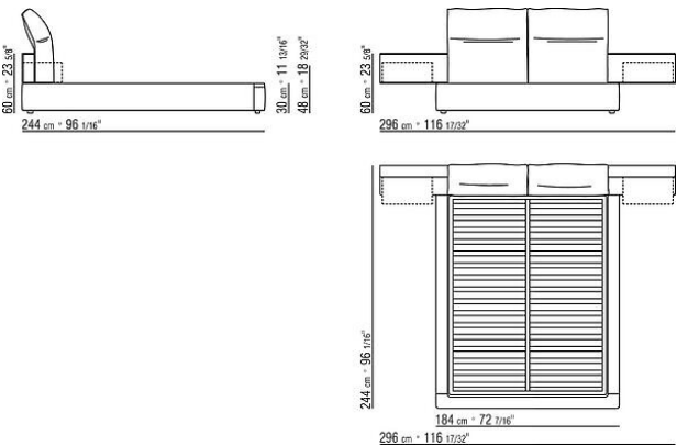
COD. 0243R1 BED W/STORAGE
