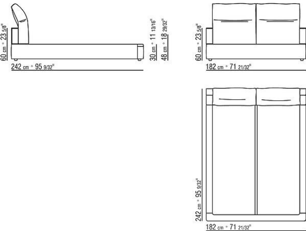
COD. 0243VA SLIM BED WITHOUT PLATFORM
