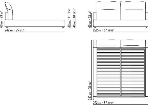
COD. 0243VE SLIM BED WITHOUT PLATFORM
