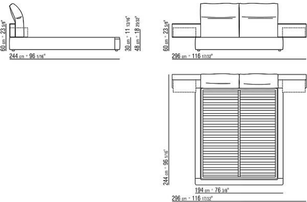
COD. 0243R2 BED W/STORAGE
