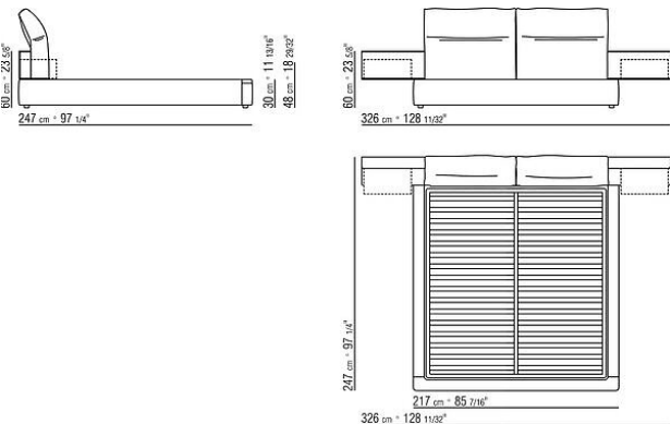
COD. 0243Q8 KING SIZE BED W/ SLATS
