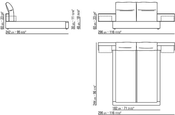
COD. 0243YA BED WITHOUT PLATFORM
