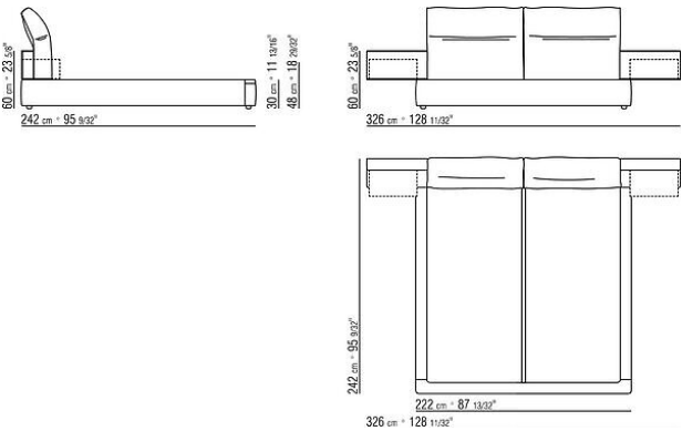
COD. 0243YE BED WITHOUT PLATFORM
