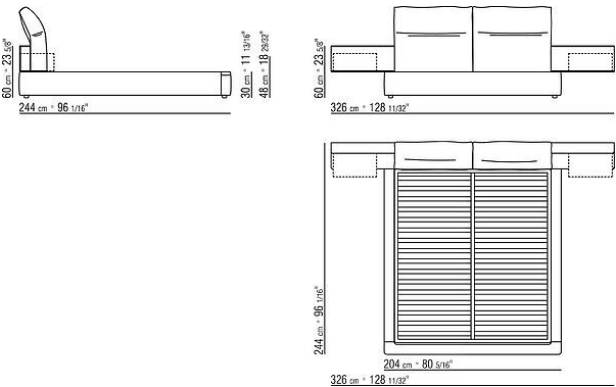
COD. 0243R3 BED W/STORAGE
