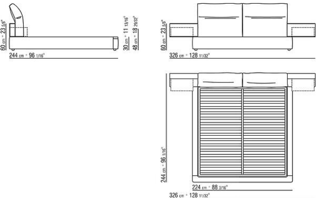
COD. 0243R5 BED W/STORAGE
