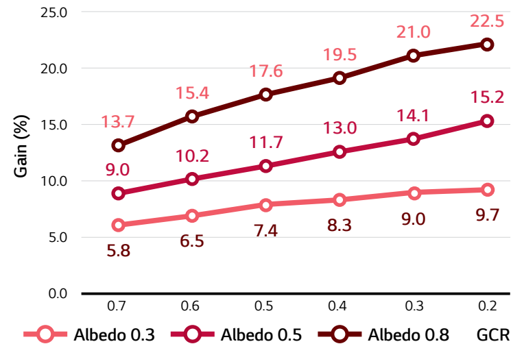
Bifacial gain by GCR
