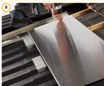
8 Mount the gutter UPPER
