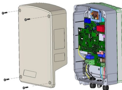
Figure 8: Opening the cover
