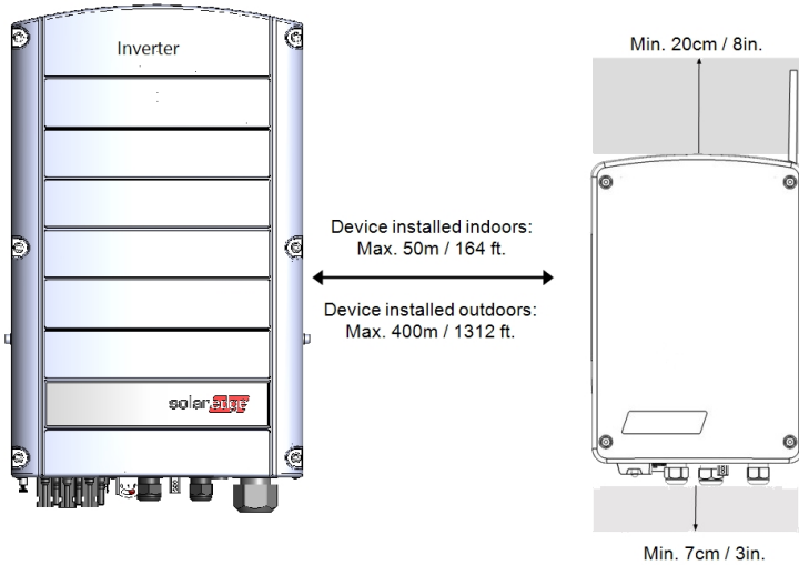
Figure 5: Clearance
