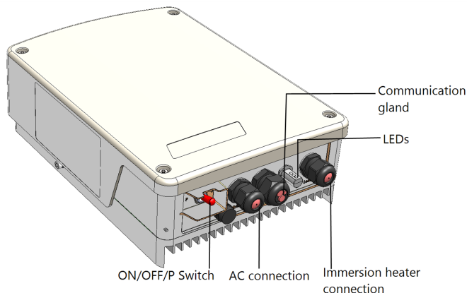
Figure 3: Device interfaces
