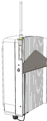
Figure 10: Mounting the Antenna
