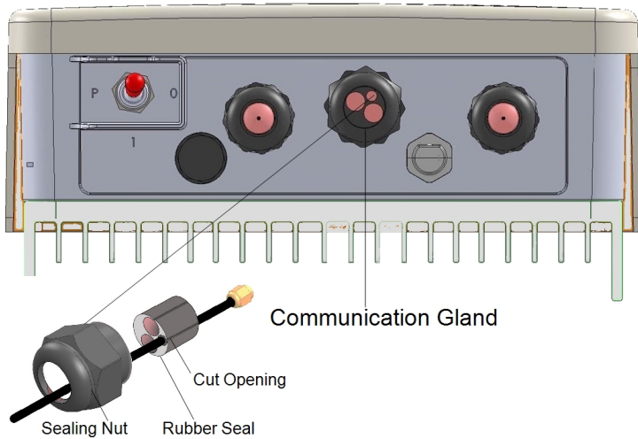
Figure 11: Communication gland
