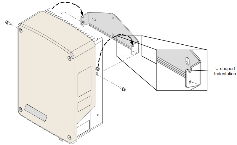
Figure 7: Hanging the device on the bracket
