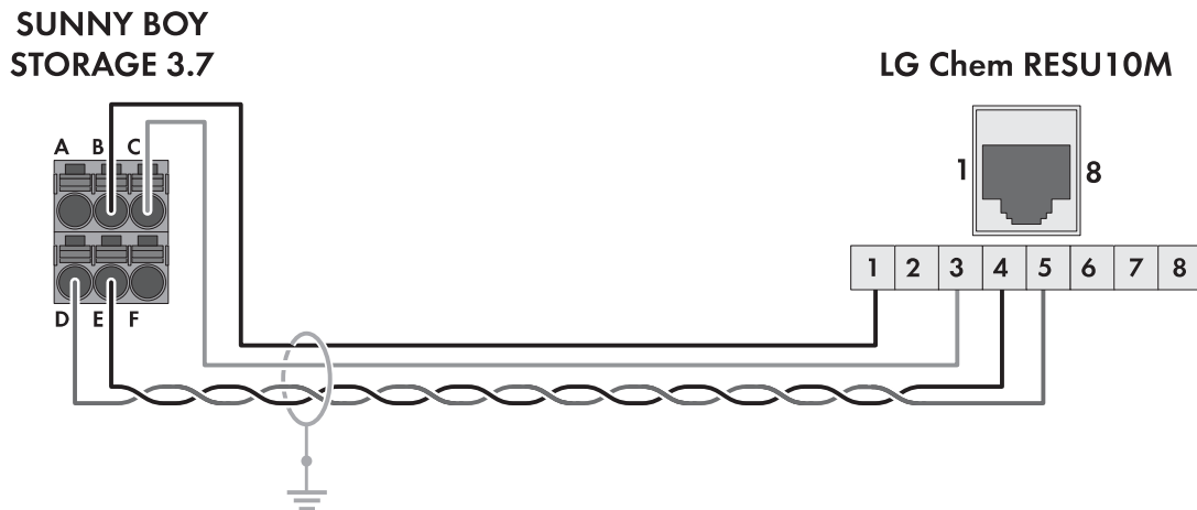
Figure 4: Cabling plan SBS3.7-10 with RESU10M
