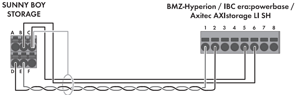
Figure 7: Cabling plan SBSxx-10 with BMZ Hyperion, IBC era:powerbase and Axitec AXIstorage Li SH
