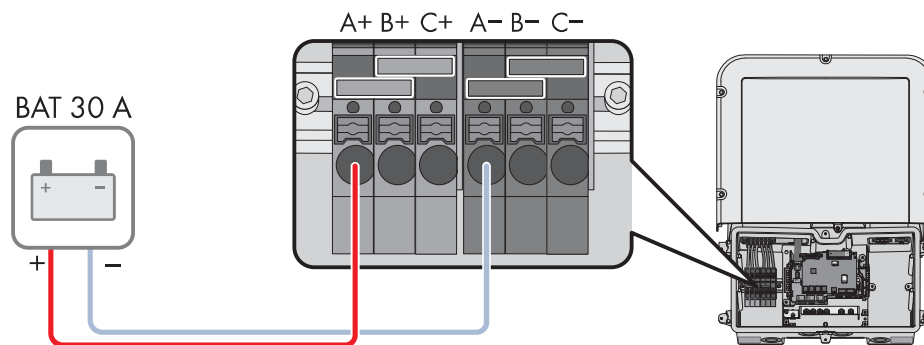
Figure 9: Overview for connection of one battery with a charging/discharging current higher than 20 A.
