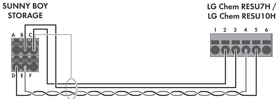
Figure 1: Cabling plan SBS2.5-1VL-10 with RESU7H / RESU10H
