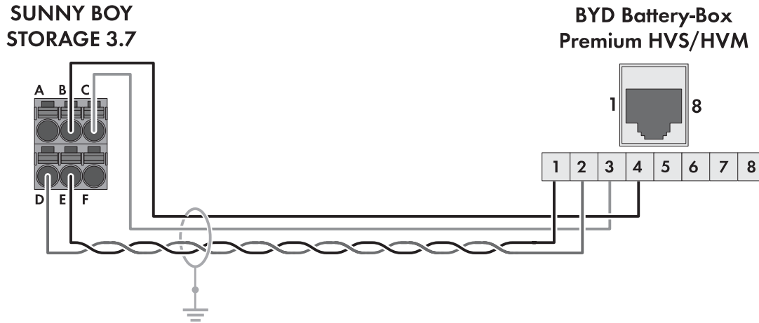
Figure 6: Cabling plan SBS3.7-10 / SBS5.0-10 / SBS6.0-10 / SBS3.8-US-10 / SBS5.0-US-10 / SBS6.0-US-10 with Battery-Box Premium HVS or HVM
