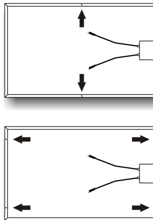
The position of holes for grounding the module – two versions (Ø4.5 mm)
