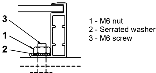
Example 2: Screwing on
