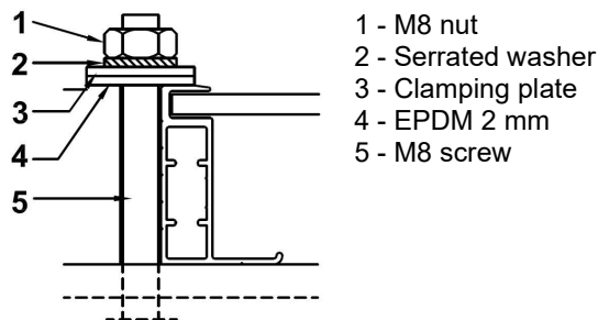
Example 1: Clamping on
