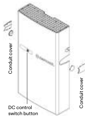
ID-behuizing
