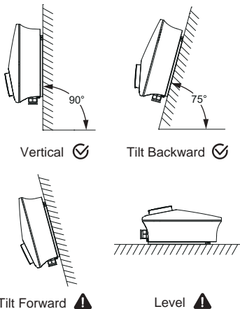
Installation Schematic Diagram
