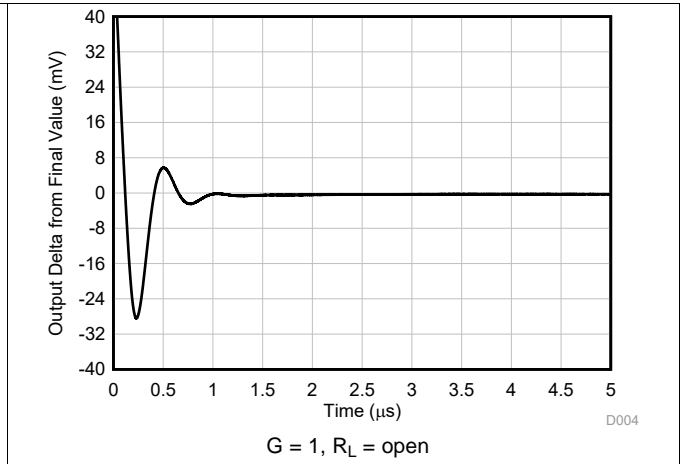
Figure 32. Large-Signal Step Response (Falling)
