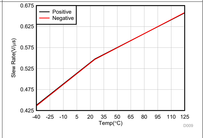
Figure 34. Slew Rate vs Temperature
