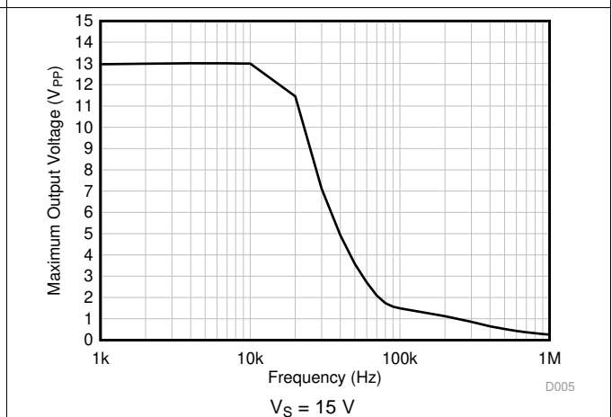
Figure 36. Maximum Output Voltage vs Frequency
