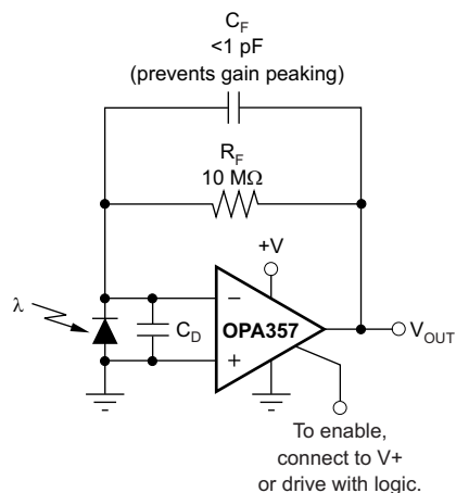
Figure 40. Transimpedance Amplifier
