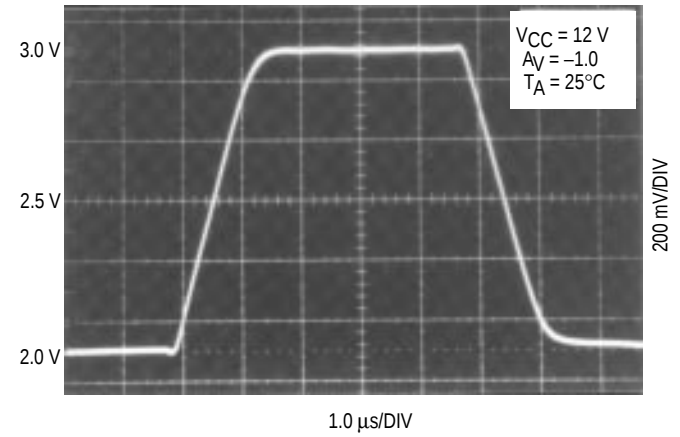
Figure 6. Error Amp Large Signal Transient Response
