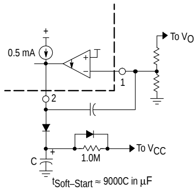
Figure 18. Soft-Start Circuit
